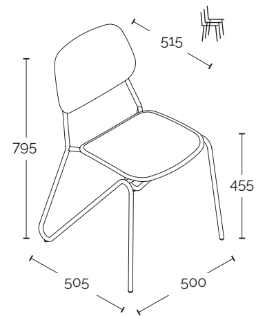
versione 4 gambe Elegance 4-leg Elegance version
